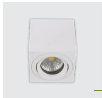
48608 Alux I. ⌀84mm ↔80mm ↗80mm aluminium-sand matt white 1xGU10/50W EAN 8585032235931 ⓐ ⓑ ⓓ
