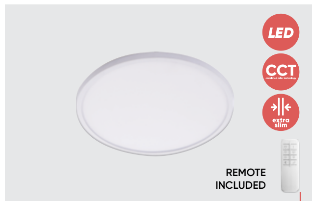
NEW 17300 Kraton I. ↓45mm Ø300mm metal, aluminium, plastic-matt white LED 18W/1490lm, 2700-6500K EAN 8585032235740 LED CCT extra slim REMOTE INCLUDED
