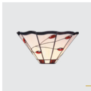
174 Tiffany III. ↓160mm ↔310mm metal-antique brown glass-tiffany 1xE14/40W EAN 8585032233654
