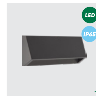
48330 Radix II. ↑70mm ↔160mm ↗33mm plastic-dark grey LED 2.9W/360lm, 4000K EAN 8585032236624 LED IP65 E A G
