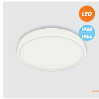
49037 Lenys II. ↓30mm Ø270mm metal-white plastic-white LED 24W/2050lm, 4000K EAN 8585032236327
