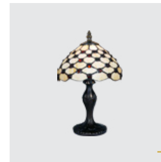
67 Tiffany VII. ⌀355mm ↔200mm ⌈200mm metal-antique brown glass-tiffany 1xE14/40W EAN 8586007084868
