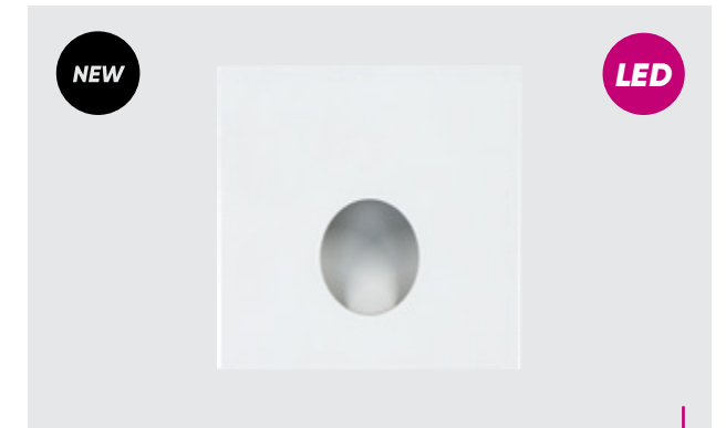
70433 Step light Olive ⚡87mm ↔87mm ↗52mm
