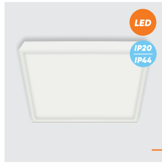
49054 Lenys SQ II. ↓25mm ↔280mm ↗280mm metal-white plastic-white LED 30W/3420lm, 4000K EAN 8585032237416
