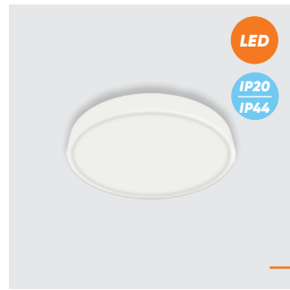
49036 Lenys II. ↓25mm Ø190mm metal-white plastic-white LED 18W/1627lm, 4000K EAN 8585032236310
